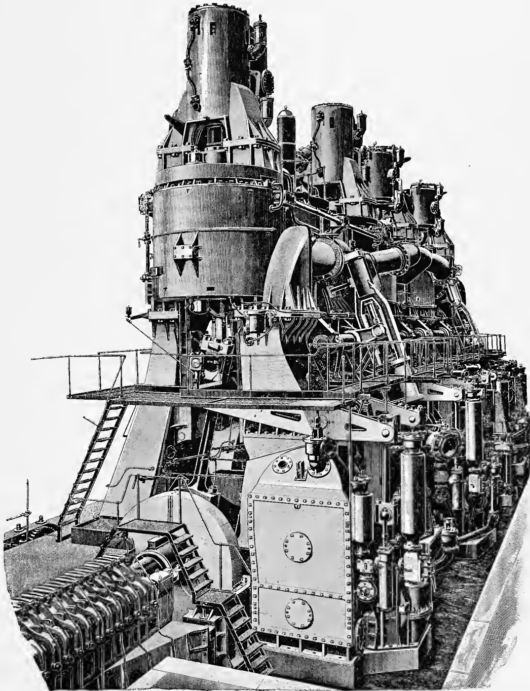
TRIPLE-EXPANSION ENGINES OF THE CAMPANIA.
